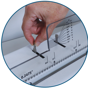
Easy Access to Punch Pins Disengage selected pins to prevent partially punched holes. No tools required.
