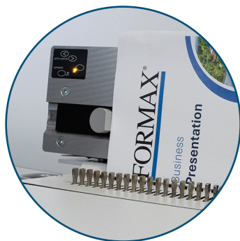
Paper Stop with Auto Sensor Activates when paper is inserted, for accurate punching
