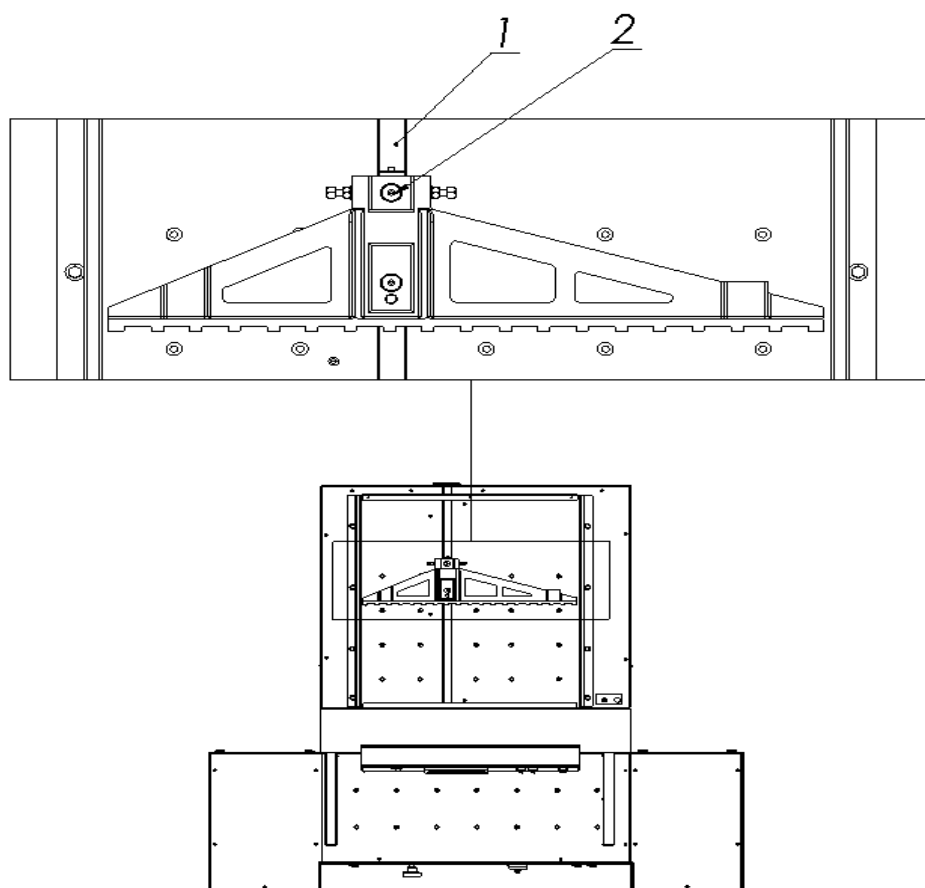
Drawing 39 Backage lubrication points location
