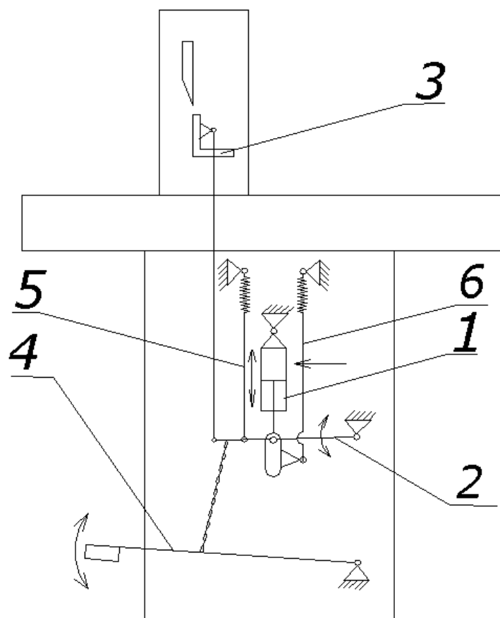
Drawing 5. Kinematic diagram for the clamping bar drive mechanism
