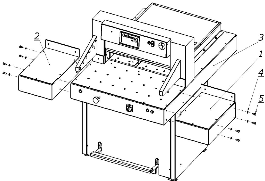
Drawing 1. Side tables installation
