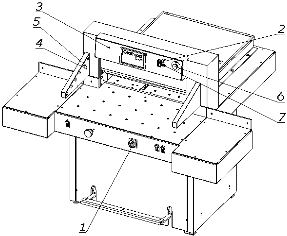
Drawing 10. Elements used when turning the cutter on
