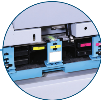
Front Access Ink Replacement 5 high-capacity 250ml ink tanks (CMYKK) are easy to access from the front, keeping the web intact
