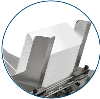
Built-In Top-Load Feeder Easily reload during print runs, features a pressure roller transport system
